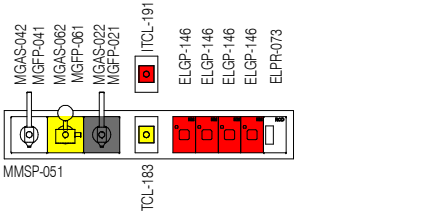
ELEVATION 8 ( 1 : 25 @ A3 )
