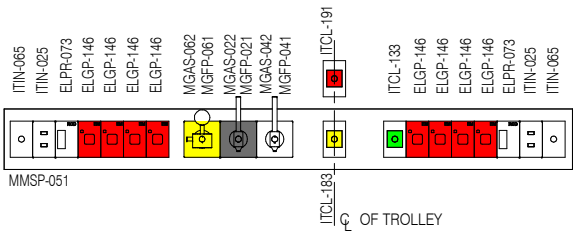
ELEVATION 5 ( 1 : 25 @ A3 )
