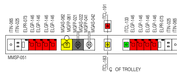
ELEVATION 5 ( 1 : 25 @ A3 )
