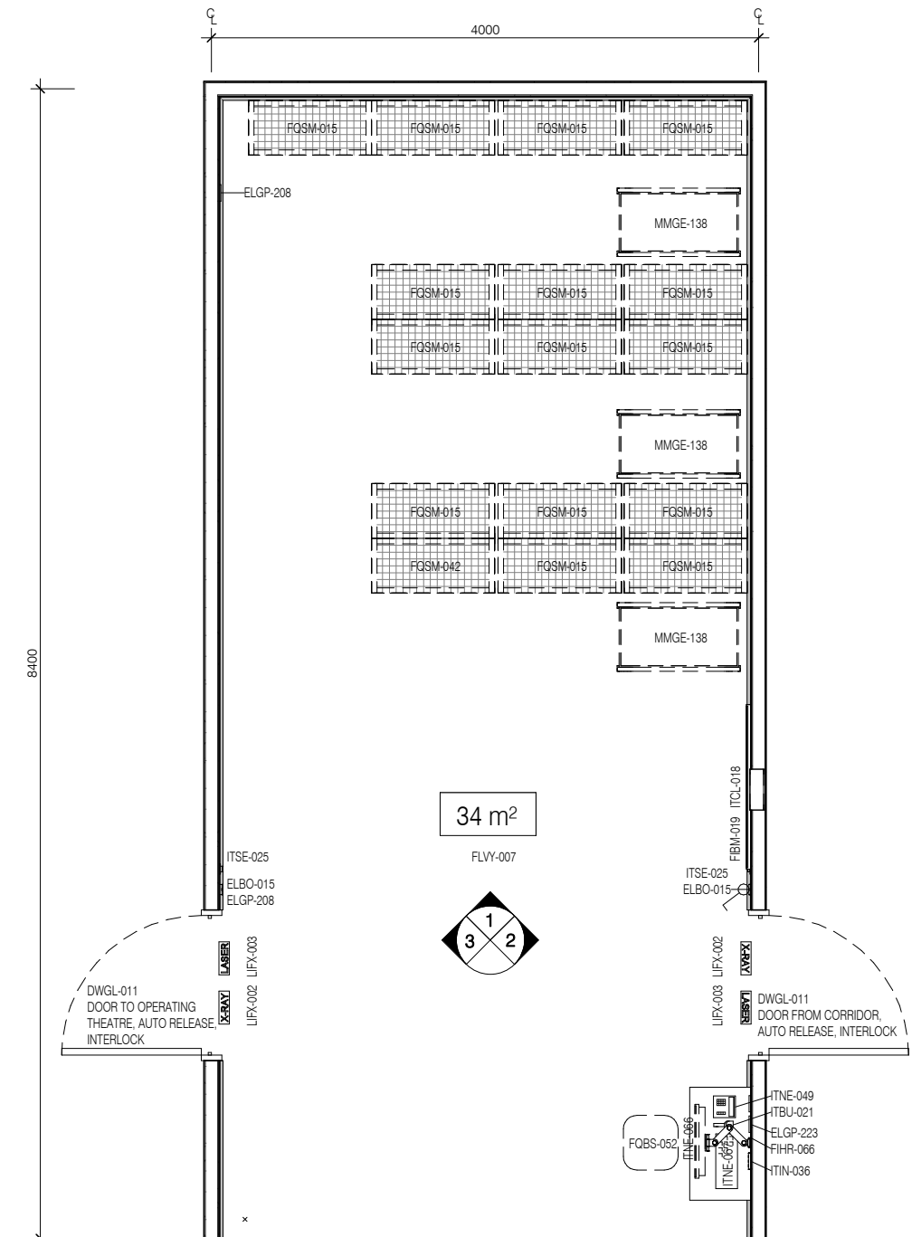
PLAN
