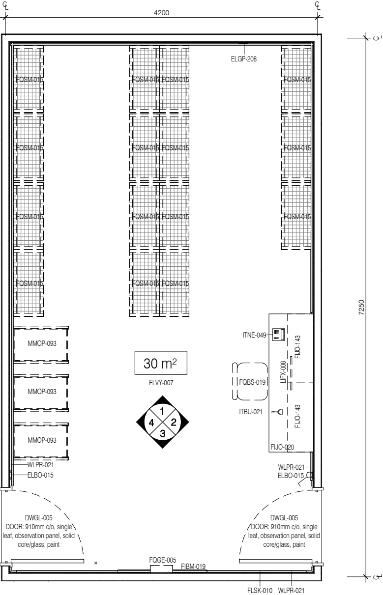
PLAN
