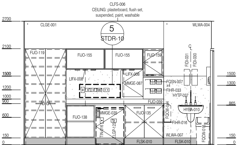
ELEVATION 5 ( 1 : 25 @ A3 )
