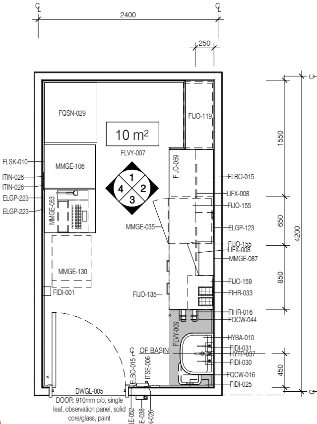
PLAN
