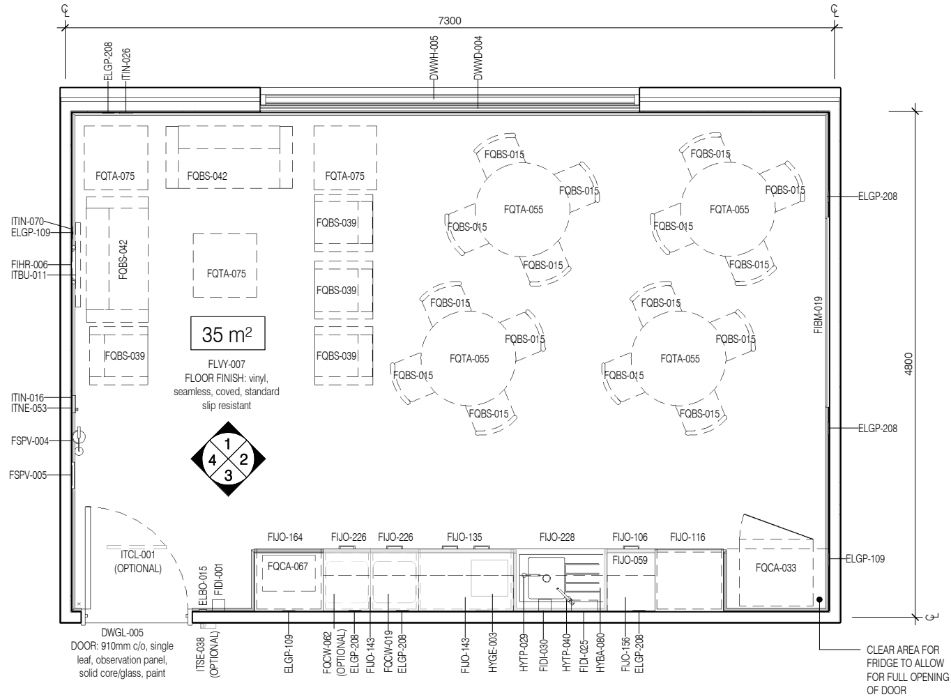
PLAN
