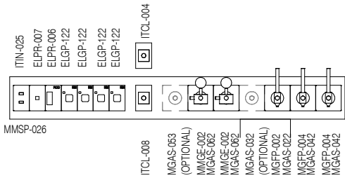
ELEVATION 5 ( 1 : 25 @ A3 )
