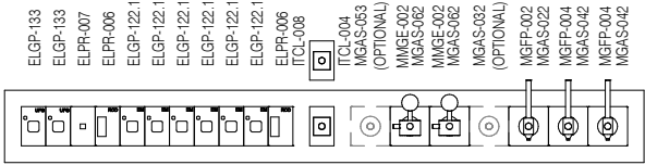
ELEVATION 5 ( 1 : 25 @ A3 )
