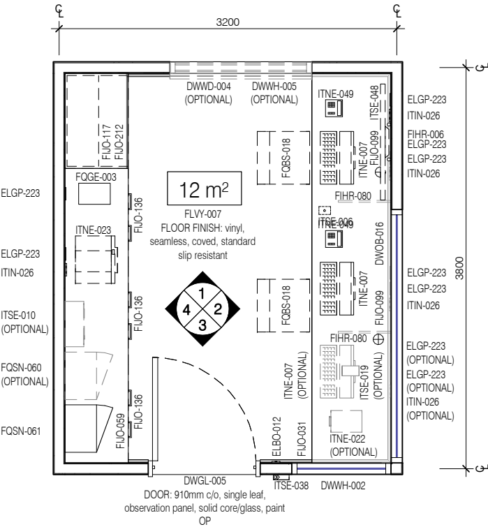
PLAN
