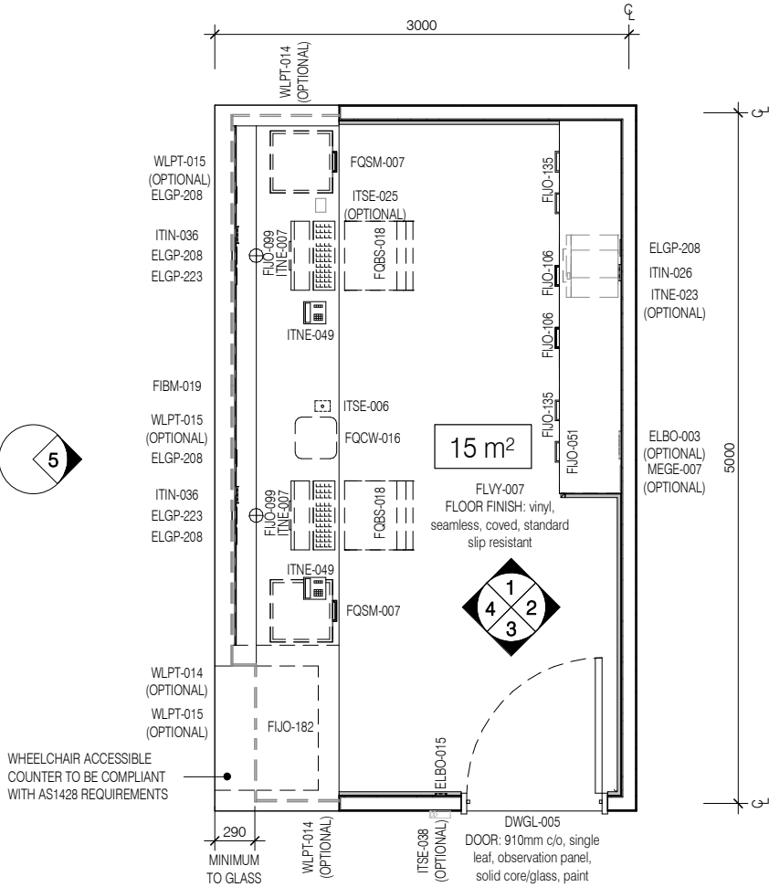
PLAN
