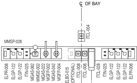
ELEVATION 3 ( 1 : 25 @ A3 )
