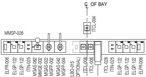
ELEVATION 3 ( 1 : 25 @ A3 )
