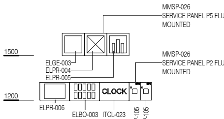
ELEVATION 5 ( 1 : 25 @ A3 )
