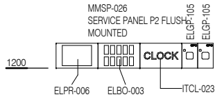
ELEVATION 5 ( 1 : 25 @ A3 )
