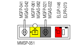
ELEVATION 7 ( 1 : 25 @ A3 )
