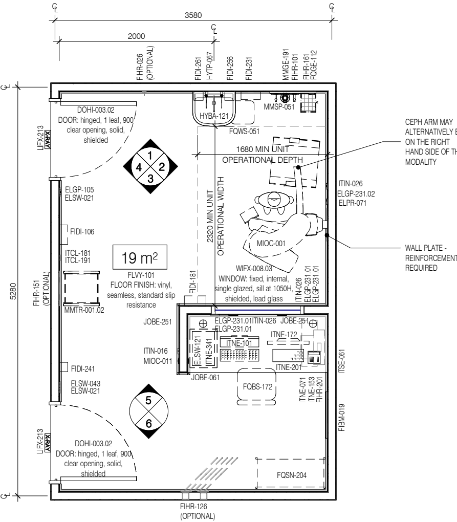
PLAN
