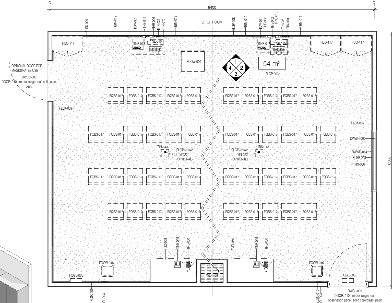
PLAN
