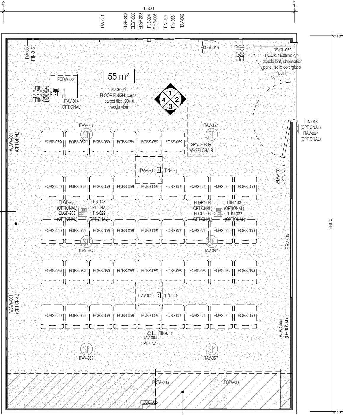
PLAN
