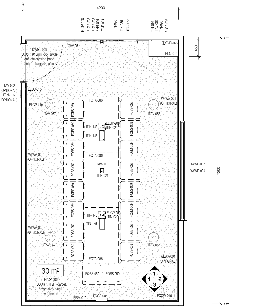
PLAN
