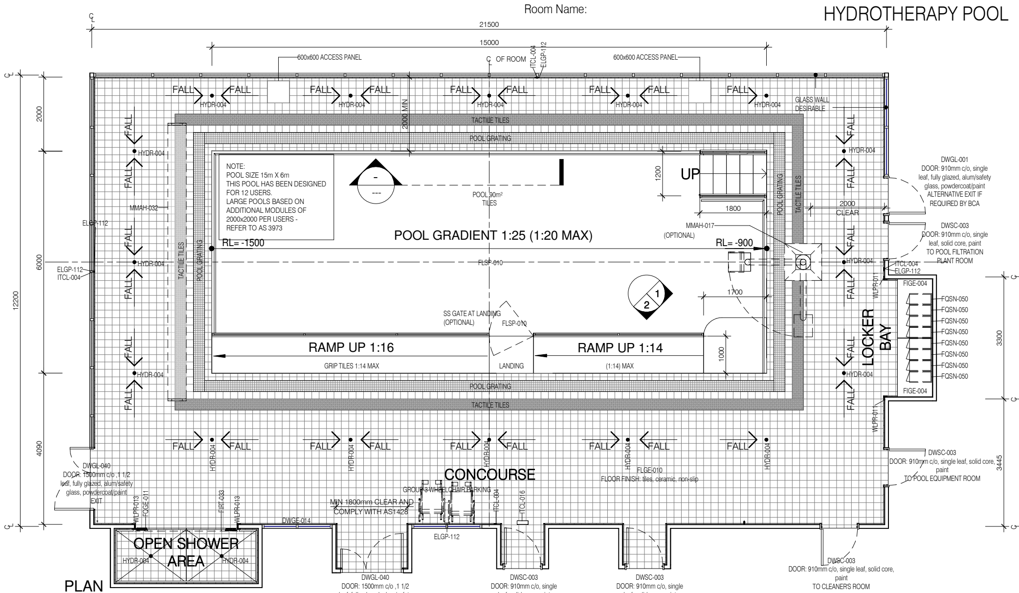
PLAN
