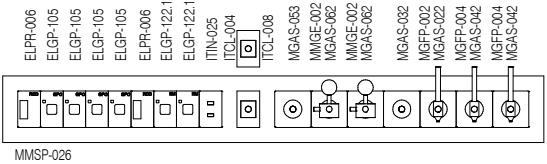
ELEVATION 5 ( 1 : 25 @ A3 )
