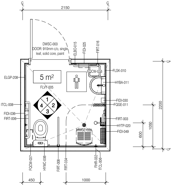
PLAN
