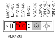
ELEVATION 6 ( 1 : 25 @ A3 )
