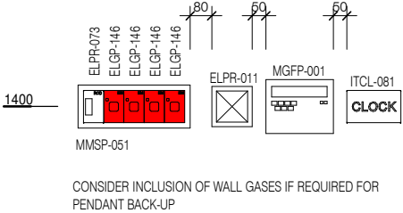
ELEVATION 5 ( 1 : 25 @ A3 )
