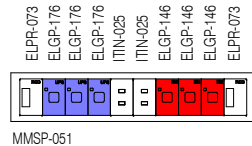
ELEVATION 7 ( 1 : 25 @ A3 )
