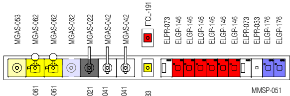
ELEVATION 5 ( 1 : 25 @ A3 )
