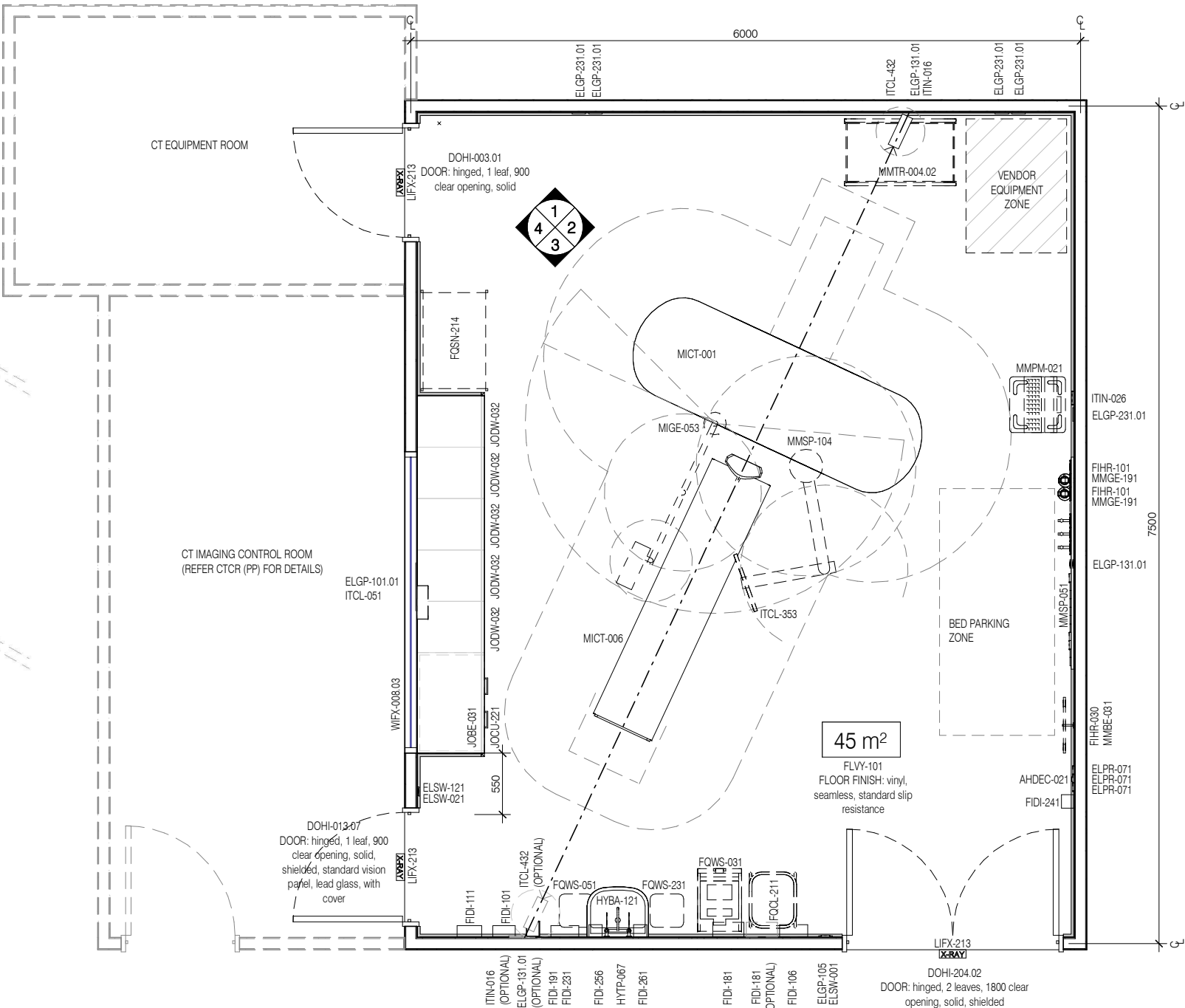
PLAN
