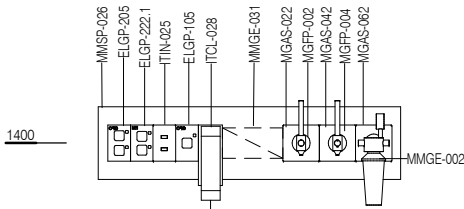
ELEVATION 5 ( 1 : 25 @ A3 )
