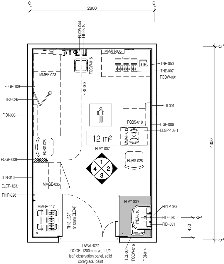
PLAN
