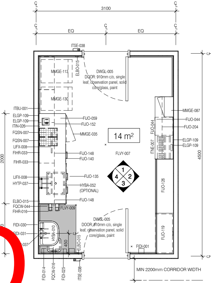
PLAN
