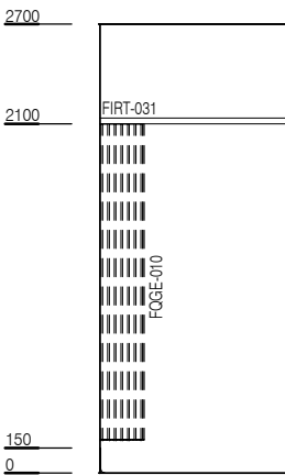
ELEVATION 4 (OPTION 3) WITH PRIVACY CURTAIN
