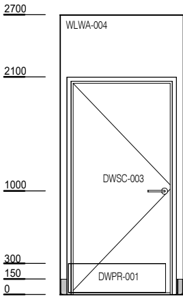
ELEVATION 4 (OPTION 1) WITH DOOR
