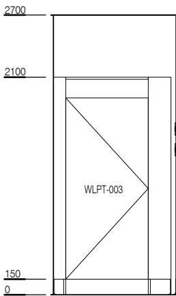
ELEVATION 4 (OPTION 2) WITH PARTITION DOOR
