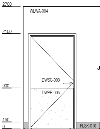
ELEVATION 4 (OPTION 1)
