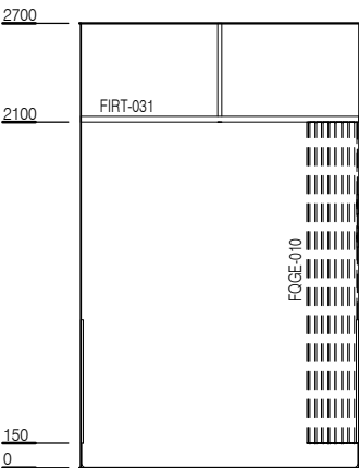
ELEVATION 4 (OPTION 3)
