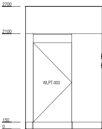
ELEVATION 4 (OPTION 2)
