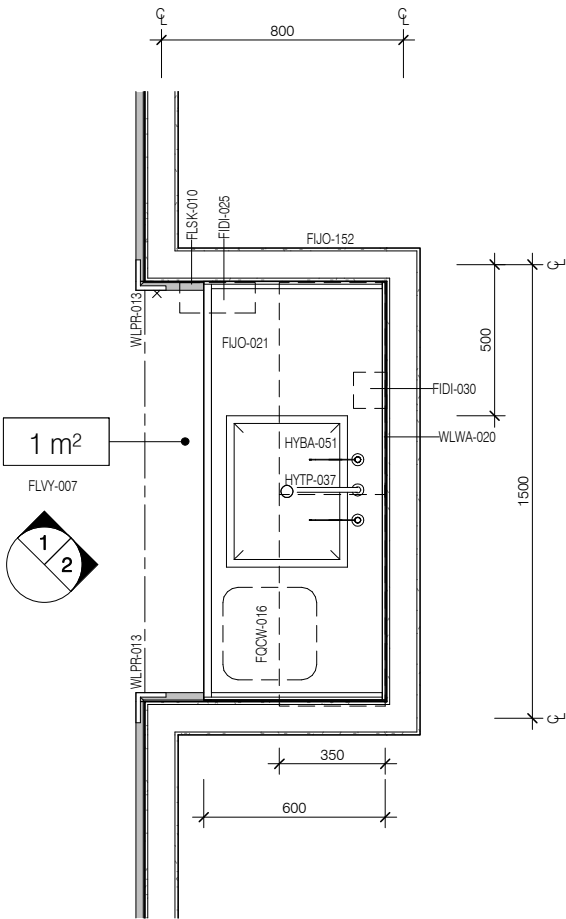
PLAN
