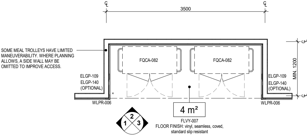
PLAN
