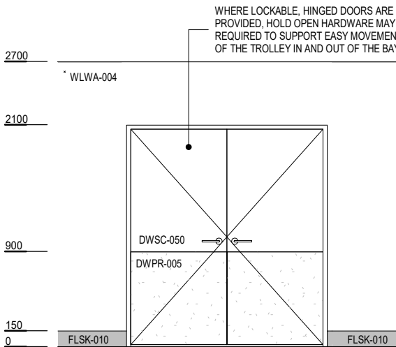
ELEVATION 2 (OPTION 2)
