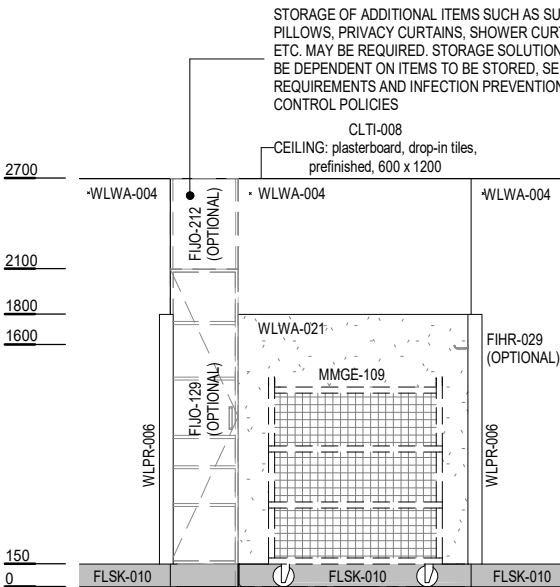
ELEVATION 2 (OPTION 1)
