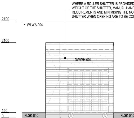
ELEVATION 2 (OPTION 3)
