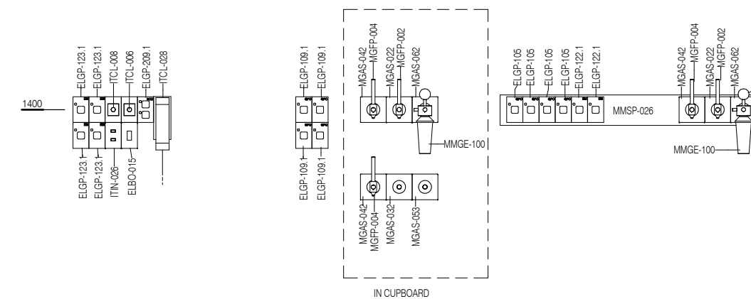
ELEVATION 6 ( 1 : 25 @ A3 )
