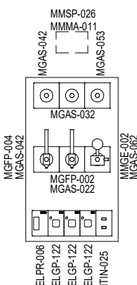
ELEVATION 7 ( 1 : 25 @ A3 )
