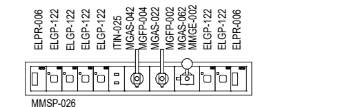
ELEVATION 6 ( 1 : 25 @ A3 )
