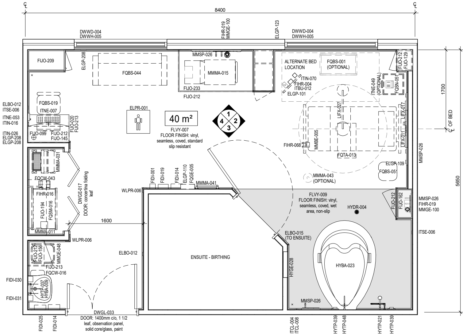
PLAN
