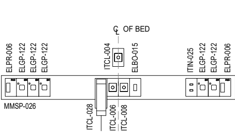
ELEVATION 7 ( 1 : 25 @ A3 )
