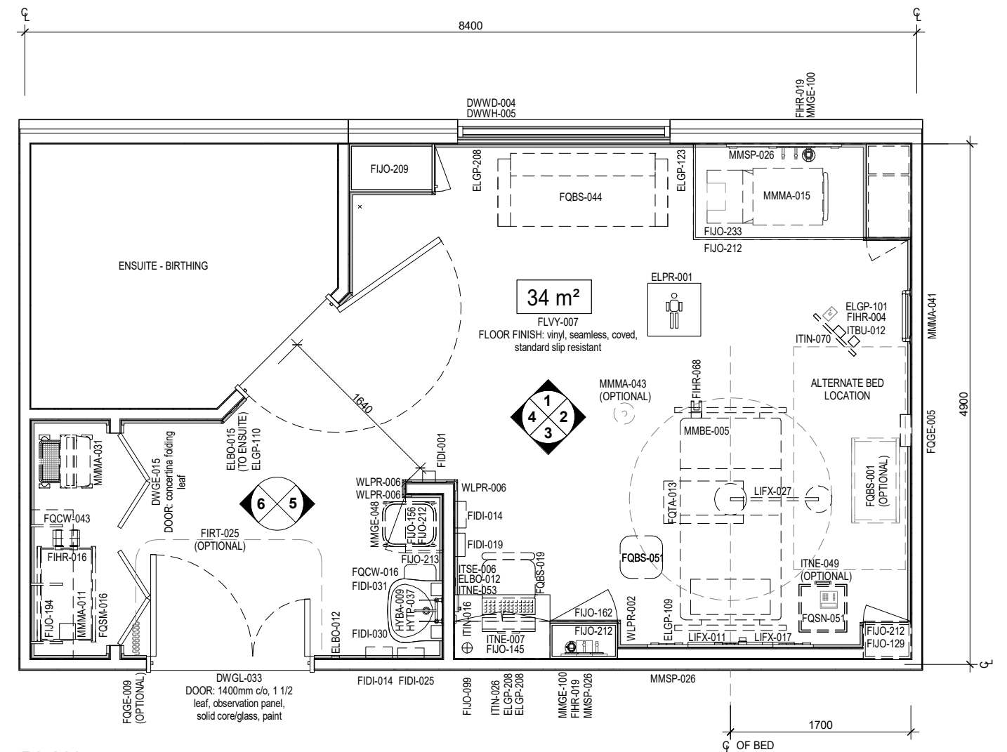
PLAN
