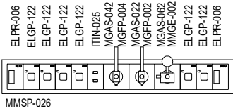
ELEVATION 8 ( 1 : 25 @ A3 ) TO RESUCITAIRE
