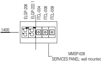
ELEVATION 6 ( 1 : 25 @ A3 )
