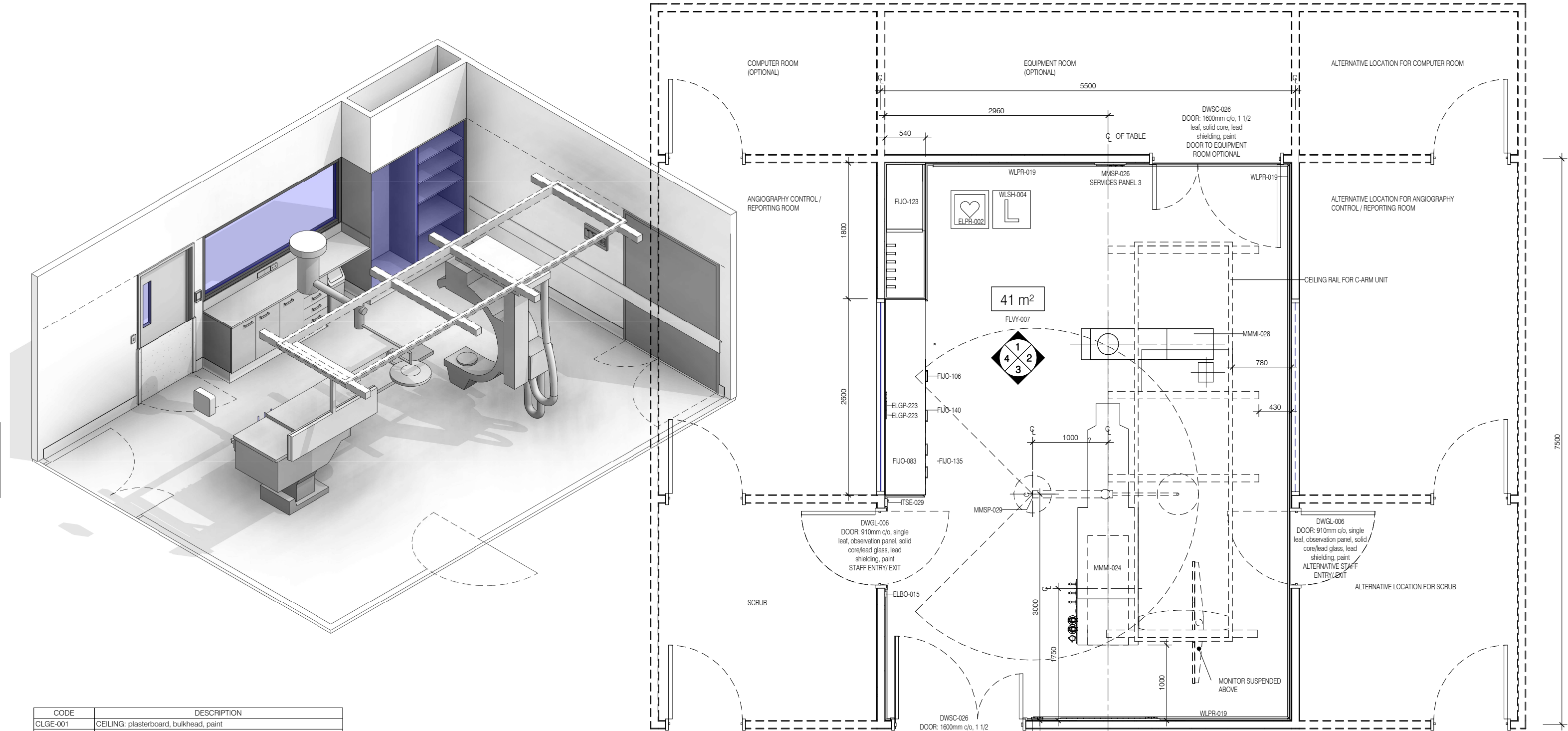
PLAN
