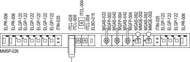
ELEVATION 5 ( 1 : 25 @ A3 )
