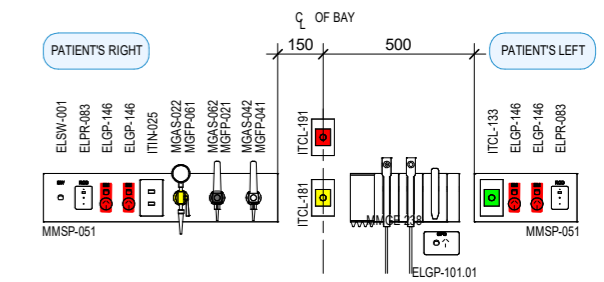
DETAIL MSP 1 (1:25 @ A3)
