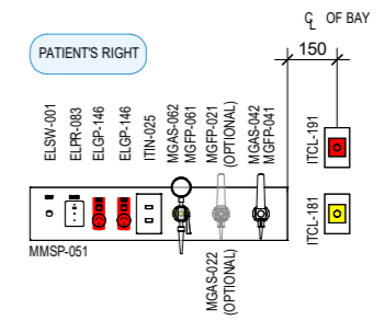
DETAIL MSP 1 (1:25 @ A3)
