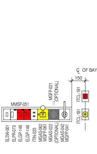
ELEVATION 4 ( 1 : 25 @ A3 )
