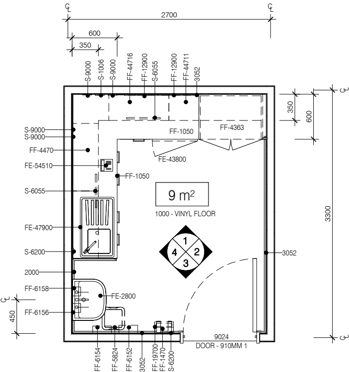
PLAN
