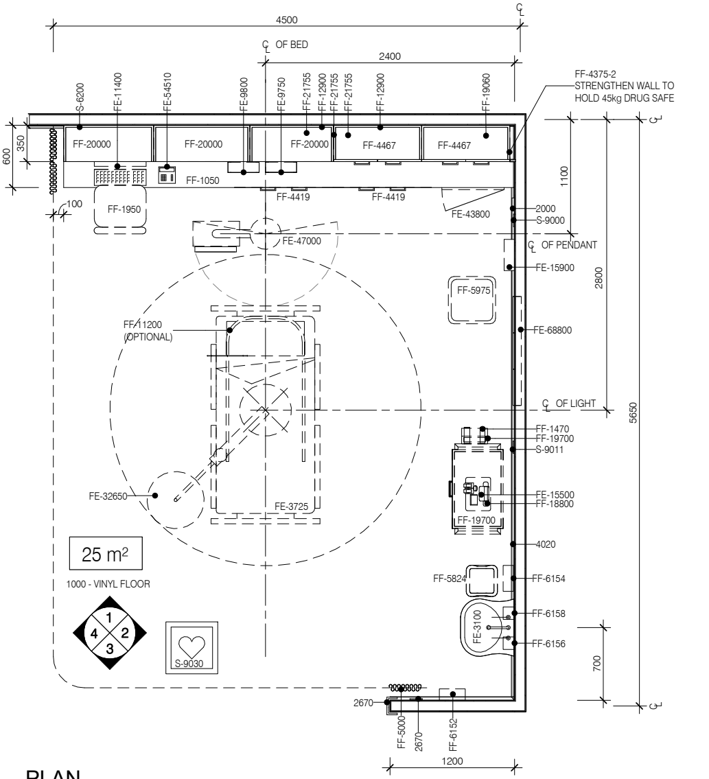
PLAN
