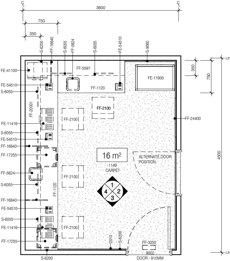
PLAN
