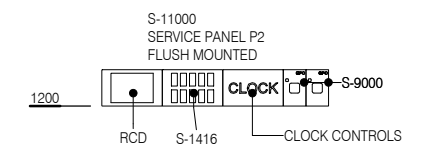
ELEVATION 5 ( 1 : 25 @ A3 )
