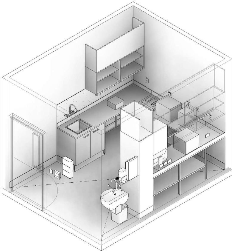
3D VIEW
