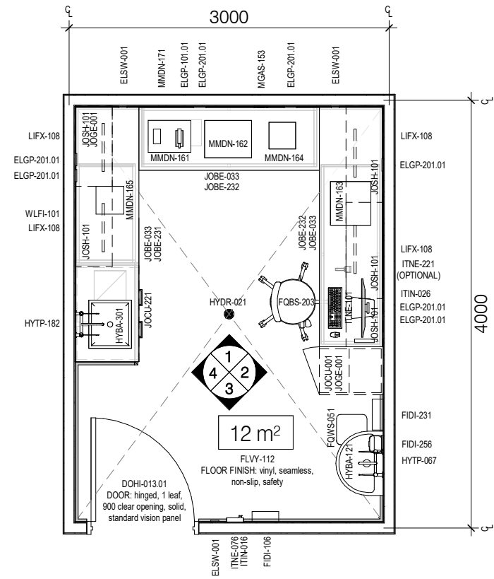
PLAN
