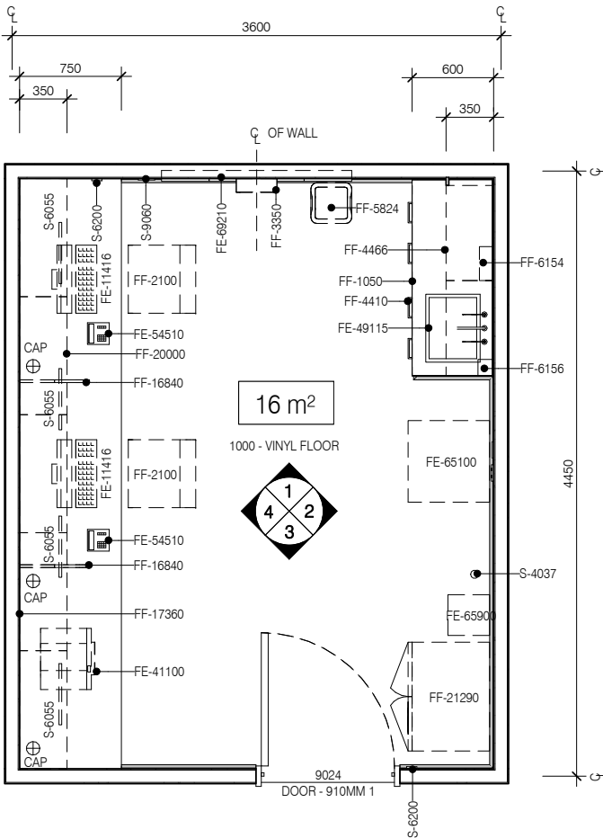
PLAN
