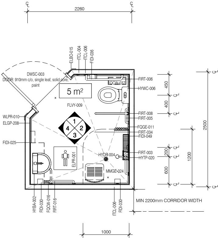
PLAN
