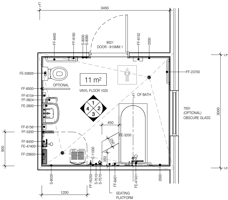
PLAN
