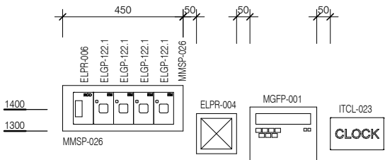
ELEVATION 5 ( 1 : 20 @ A3 )
