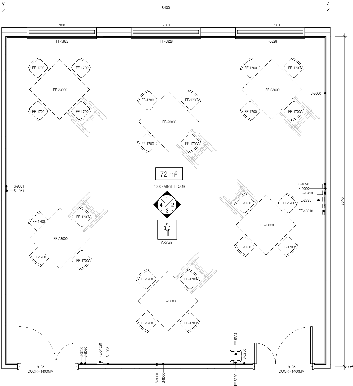
PLAN
