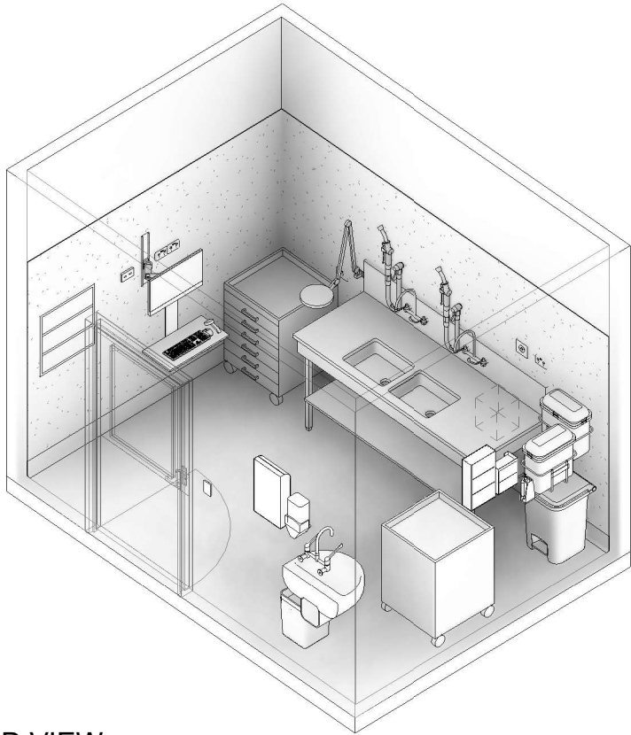
3D VIEW
